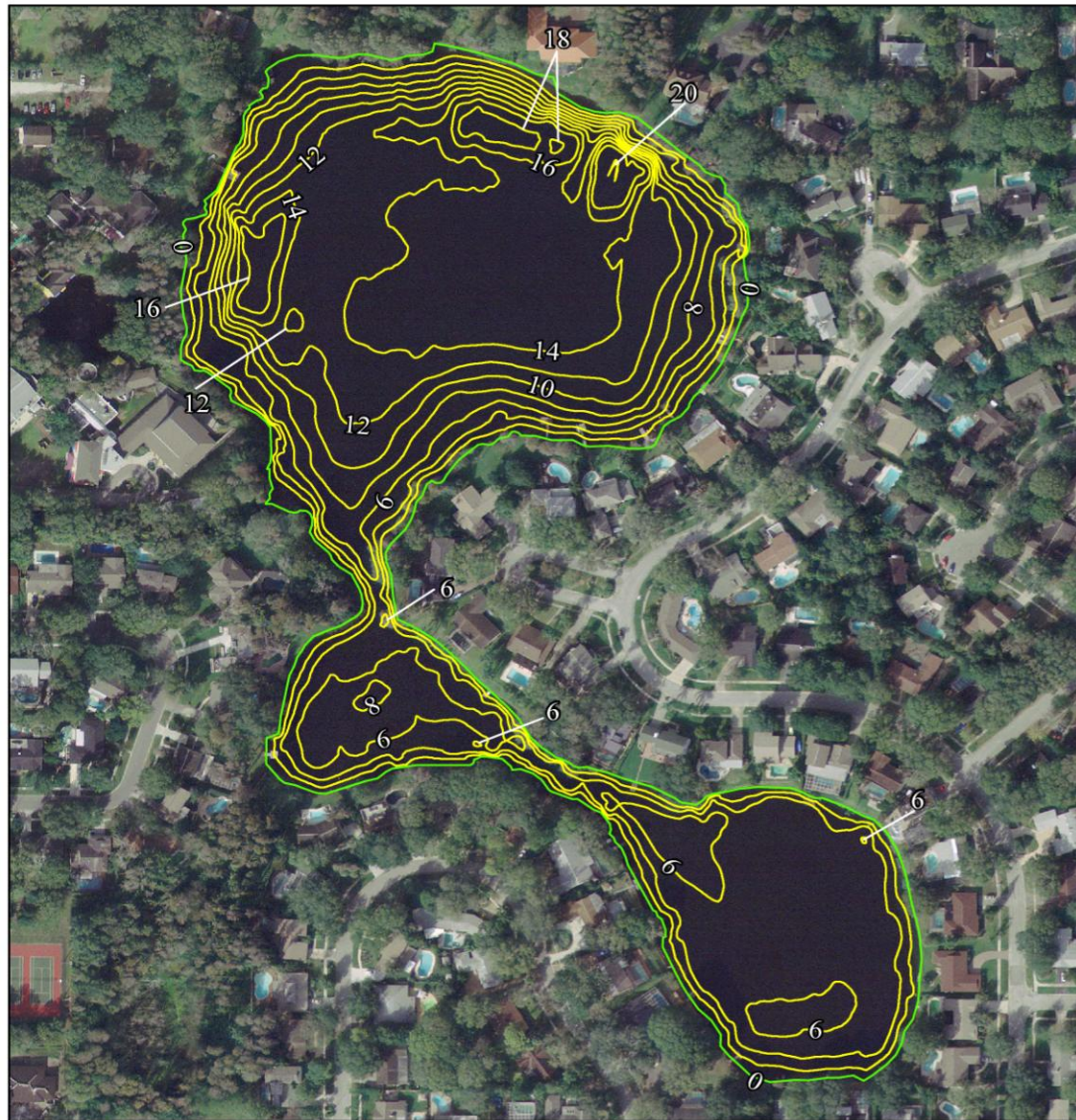
Figure 1. Contour map for Lake Lipsey. The mapping technique used in 2008 employs a standard DGPS for horizontal position and a fathometer for depth.
