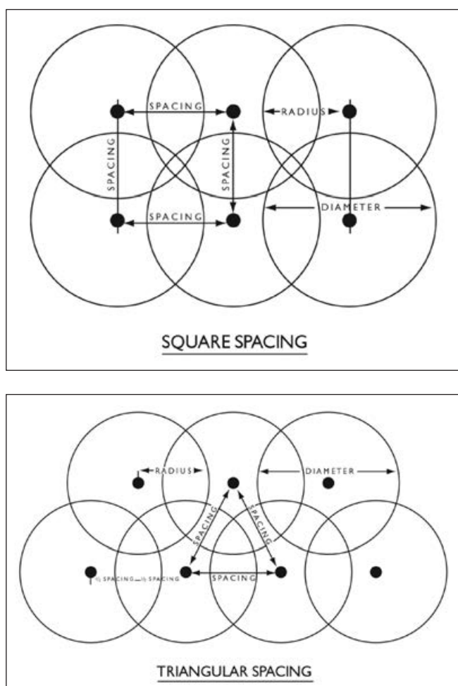
Figure 5. Sprinkler layouts.
