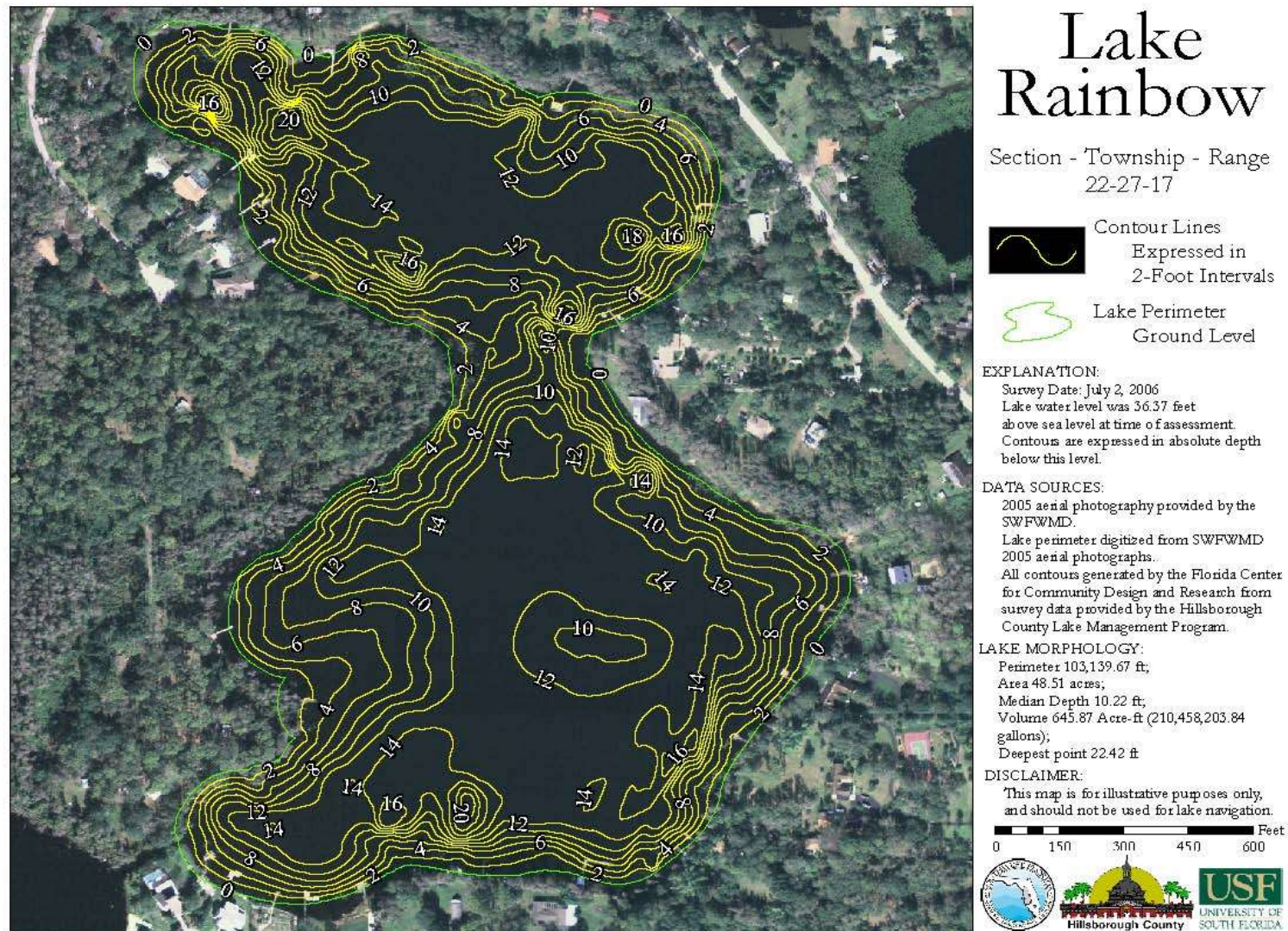
Figure 2. Rainbow Lake Bathymetric Contour Map
