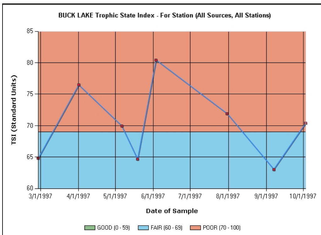
Figure 6. Recent Trophic State Index (TSI) graph from Hillsborough Watershed Atlas. For the latest date go to: ( http://www.hillsborough.wateratlas.usf.edu/lake/waterquality.asp?wbodyid=5129&wbodyatlas=lake )
