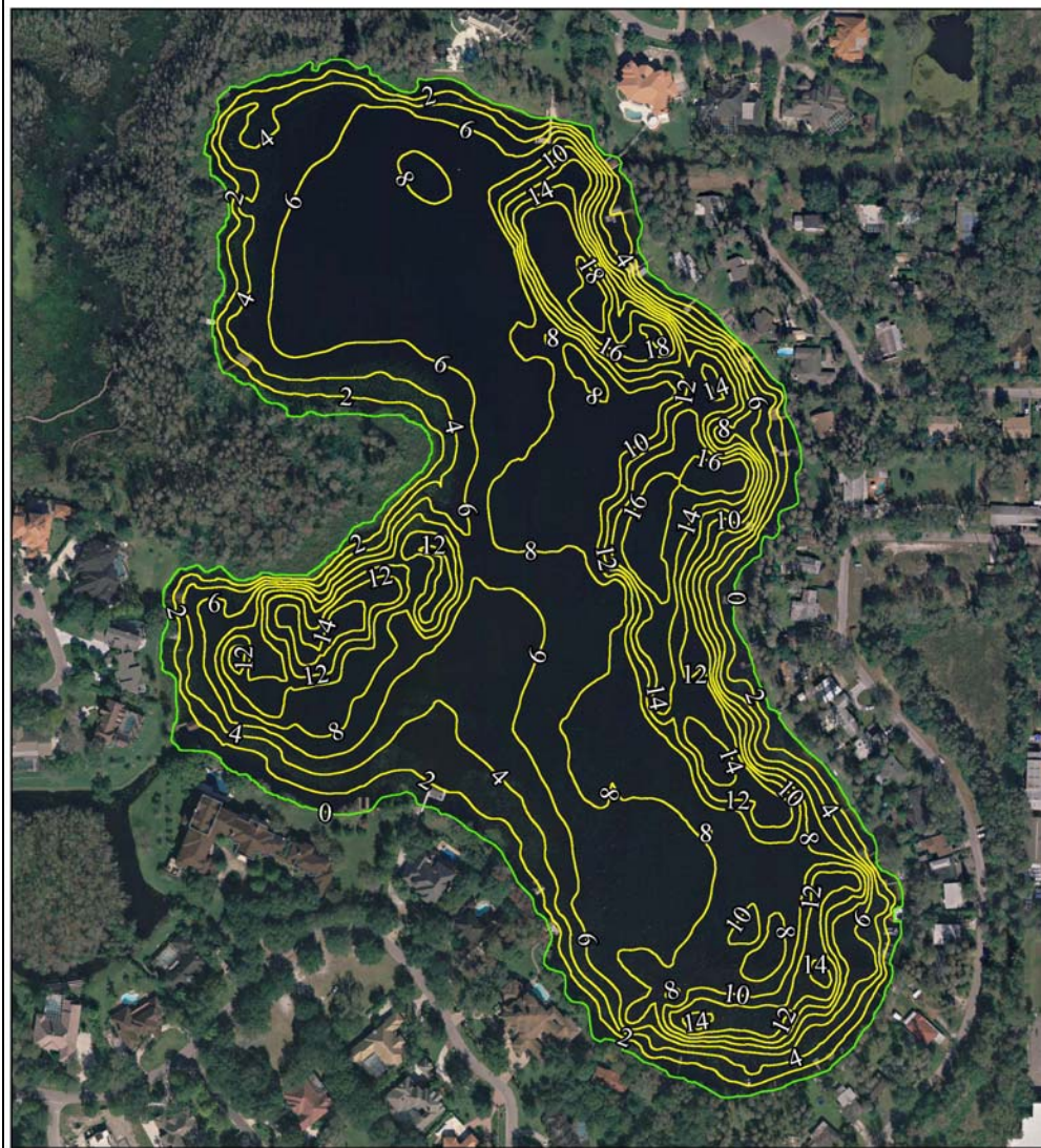
Figure 2. Contour map for Chapman Lake. The mapping technique used in 2007 employs a standard DGPS for horizontal position and a fathometer for depth.
