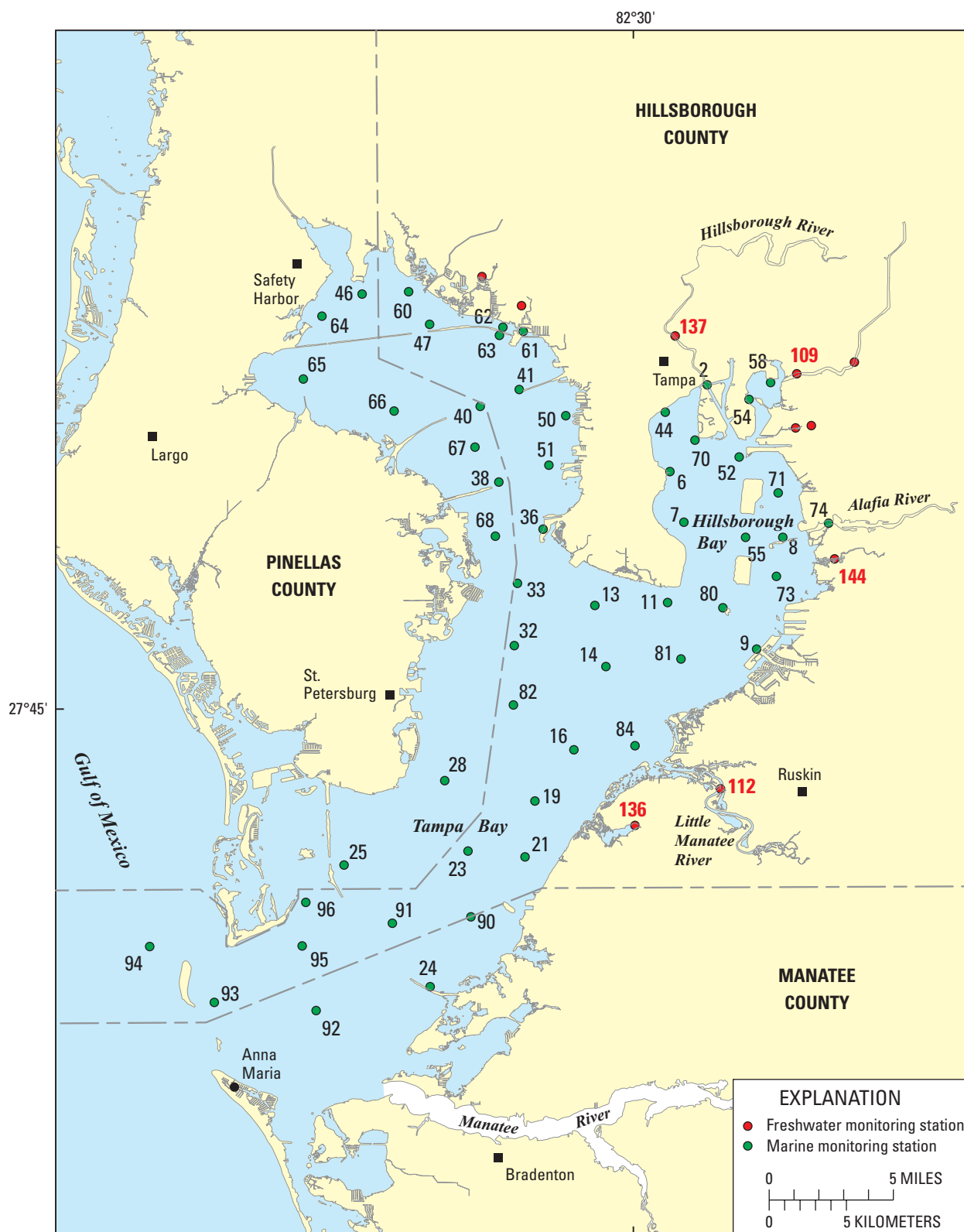
Figure 5-12. Environmental Protection Commission of Hillsborough County water-quality stations in Tampa Bay. From Environmental Protection Commission of Hillsborough County.
