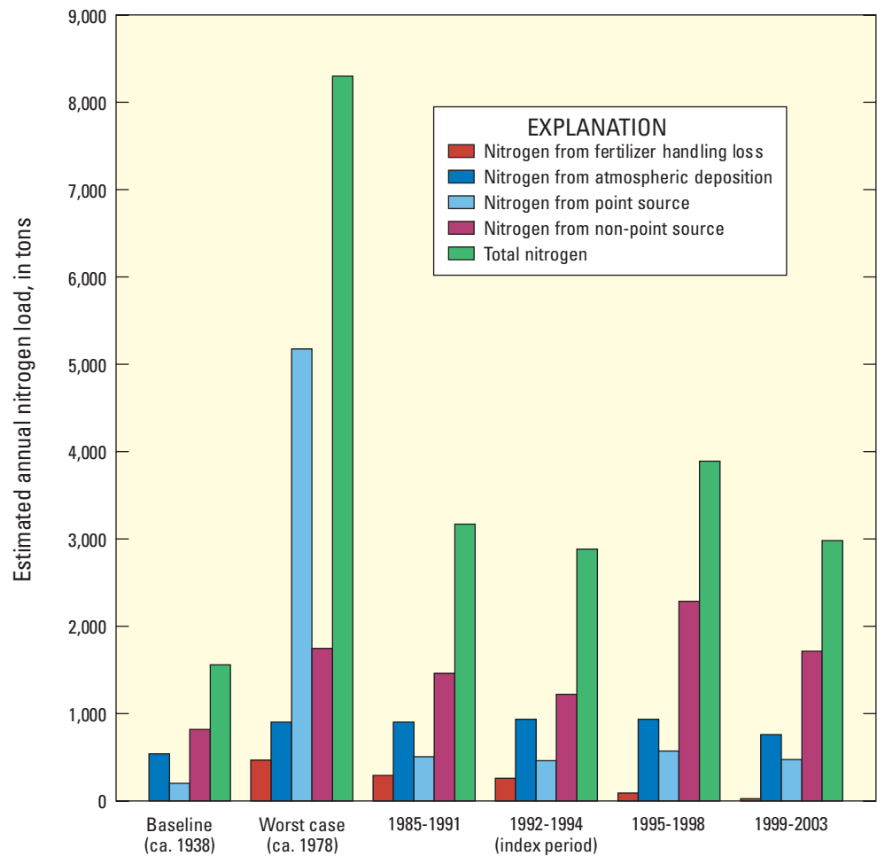
Figure 5-16. Estimated annual nitrogen loads to Tampa Bay during various time periods (1938–2003). Data from Janicki Environmental, Inc. (2008) and Greening and Janicki (2006).
