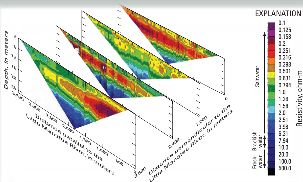
Box 5-1, Figure 2. Three dimensional resistivity profile taken near the Little Manatee River located on the eastern shoreline of Middle Tampa Bay. Axes indicate position of the transect relative to the river mouth. Dark blue colors indicate fresh and brackish water, green and red colors indicate saltier water. Depth (in meters) is the depth below the bay floor.
