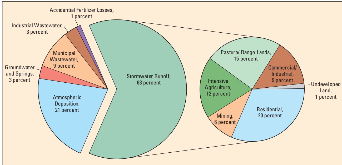
Figure 5-21. Sources of total nitrogen to Tampa Bay, 2003–2007 (Janicki Environmental Inc. (2008).
