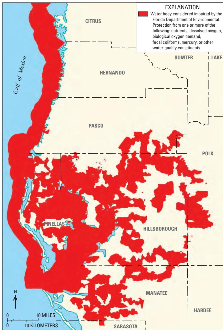
Figure 5–11. Impaired waterbodies within the Tampa Bay watershed, 2009. Red areas are considered impaired for one or more of the following: nutrients, dissolved oxygen, biological oxygen demand, fecal coliforms, mercury or other water-quality constituents. From Florida Department of Environmental Protection.
