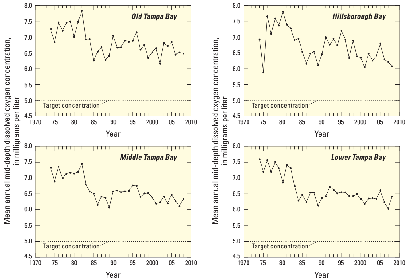
Figure 5-10. Average annual mid-depth dissolved oxygen concentrations, 1974–2008, for Hillsborough Bay, Old Tampa Bay, Middle Tampa Bay and Lower Tampa Bay. Horizontal lines depict State criteria for daily average dissolved oxygen concentrations. Data from Environmental Protection Commission of Hillsborough County.
