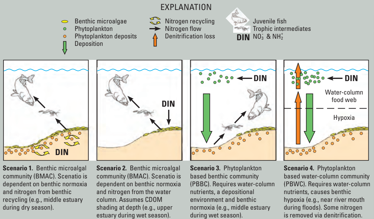
Box 8–3, Figure 2. Schematic illustrating four nitrogen (N) pathway scenarios for tidally influenced systems in Tampa Bay. From Tampa Bay Tidal Tributary Research Team (2008).
