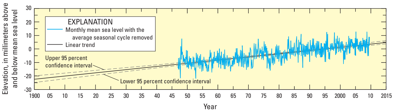
Figure 8–18. Mean sea-level trend for St. Petersburg, Florida, 1948–2009. The mean sea-level trend is 2.36 millimeter per year (mm/yr) with a 95 percent confidence interval of \pm 0.29 mm/yr based on monthly mean sea-level data from 1947 to 2006, which is equivalent to a change of 0.77 feet in 100 years. Accessed at http://tidesandcurrents.noaa.gov/sltrends/sltrends_station.shtml?stnid=8726520 .
