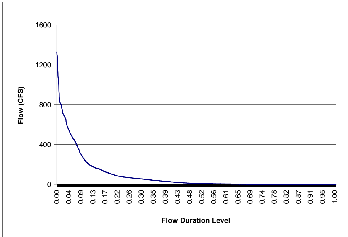
Figure 5.2. Flow Duration Curve for USGS Gage 02303800
