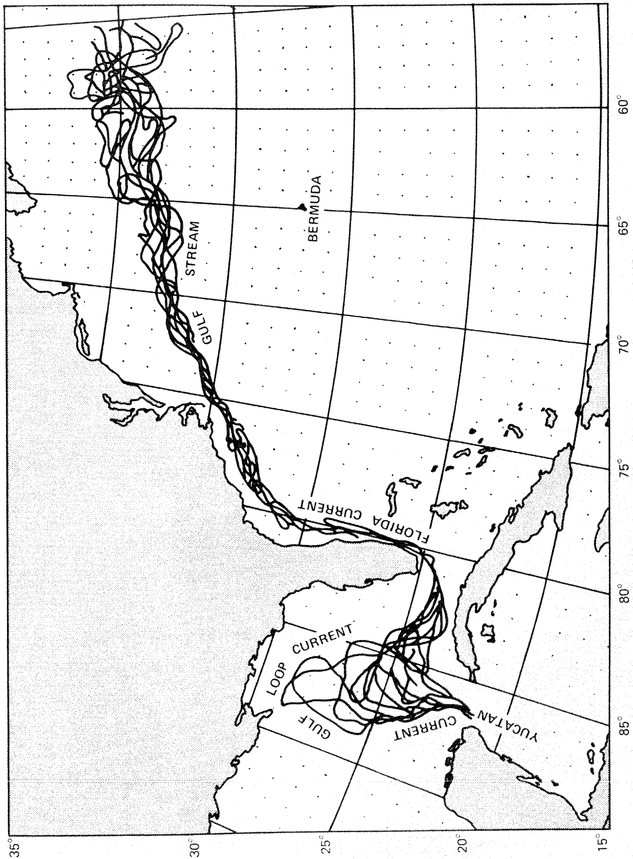
Figure 12. Components of the Gulf Stream System (Maul 1976).
