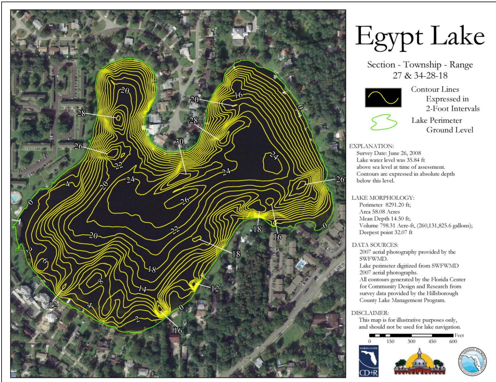
Figure 1. Contour map for Egypt Lake. The mapping technique used in 2008 employs a standard DGPS for horizontal position and a fathometer for depth.
