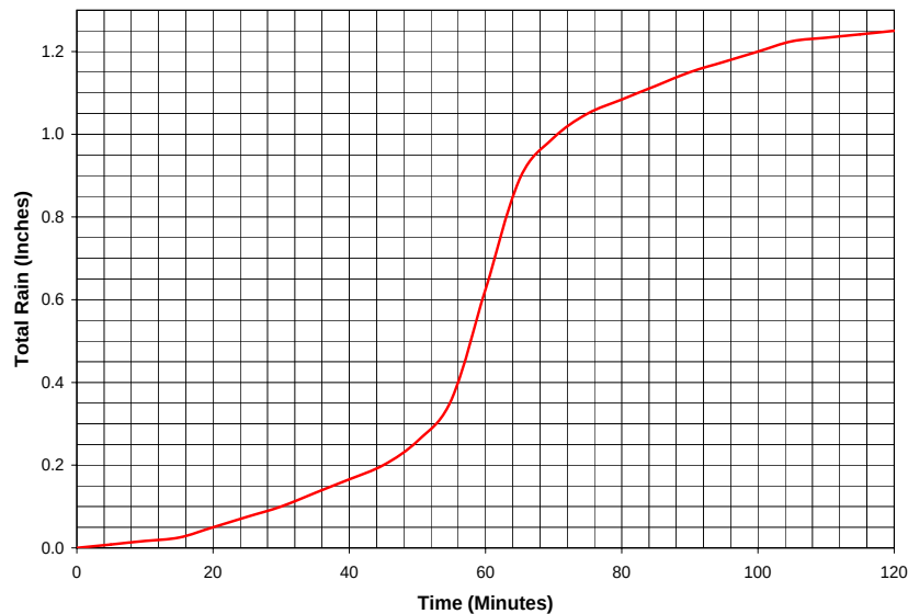
Figure 10-14: New Jersey 1.25-Inch/2-Hour Stormwater Quality Design Storm Distribution
