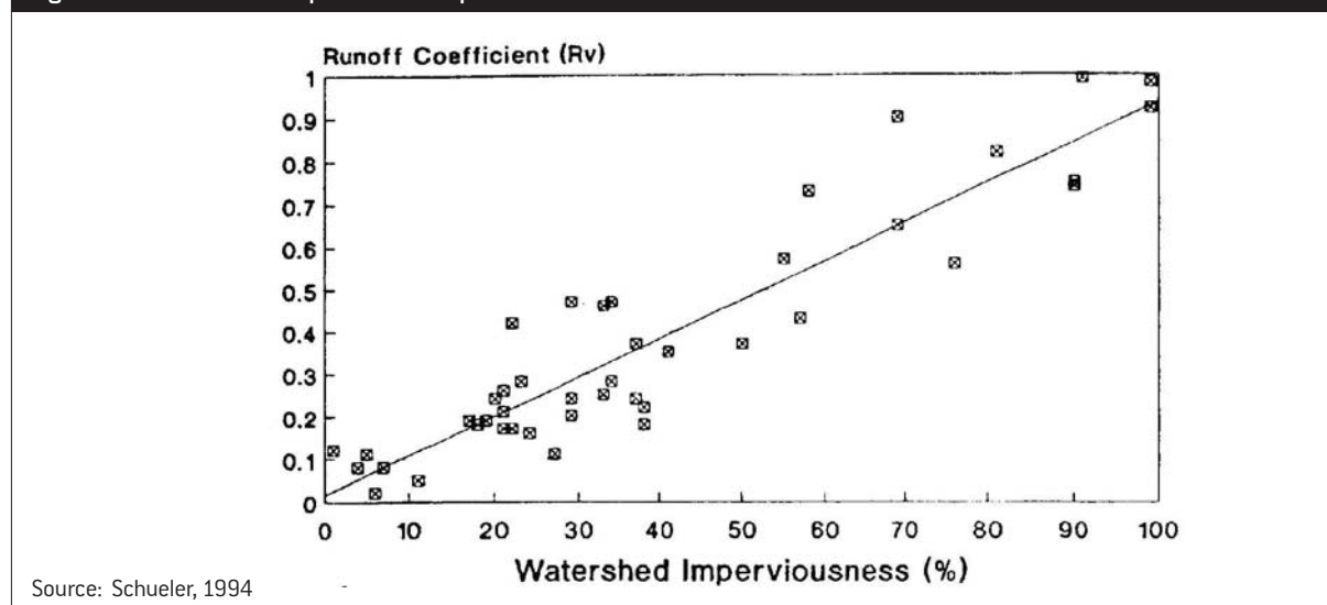
Figure 4-3: Relationship Between Imperviousness and Stormwater Runoff
