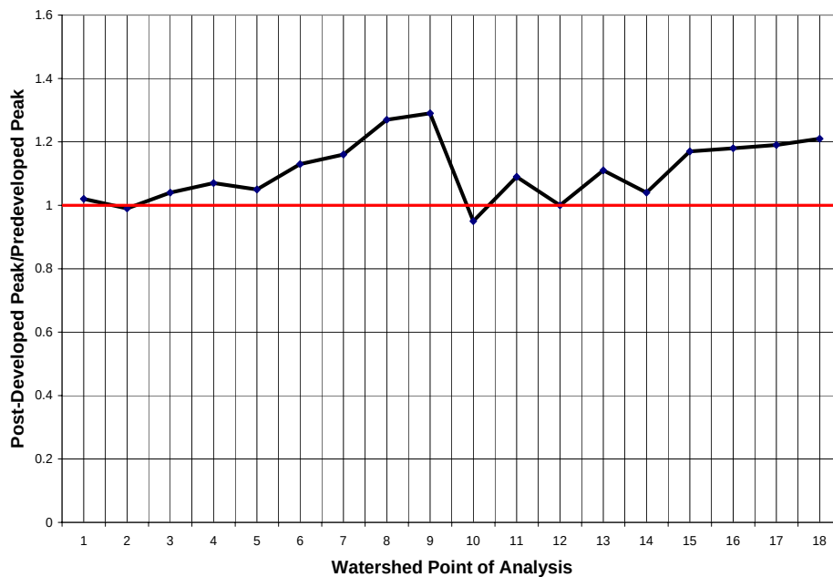
Figure 10-5: Comparison of 100-Year Pre- and Post-Developed Peak Rates with Peak Rate Controls, Devils Brook Watershed
