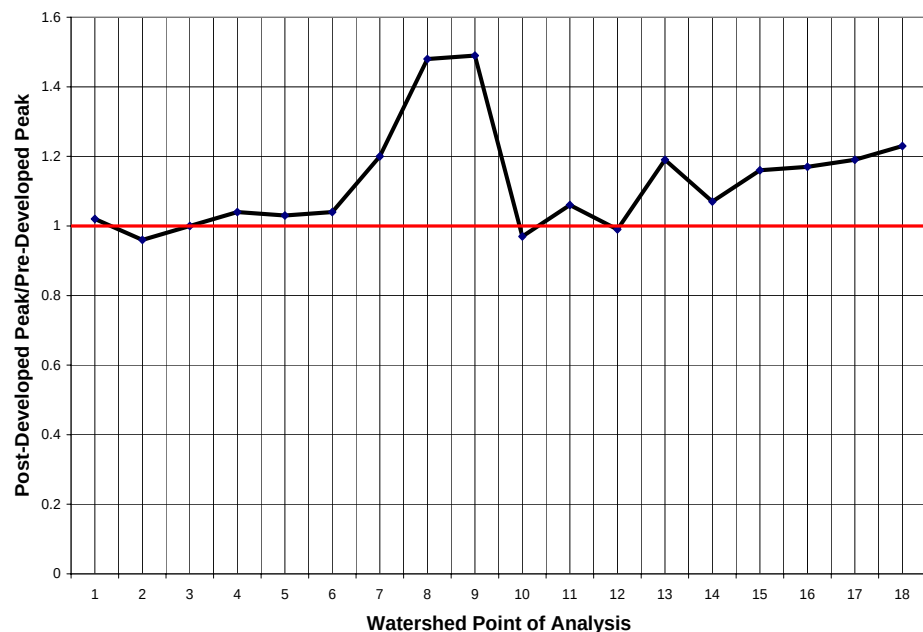
Figure 10-4: Comparison of 10-Year Pre- and Post-Developed Peak Rates with Peak Rate Controls, Devils Brook Watershed
