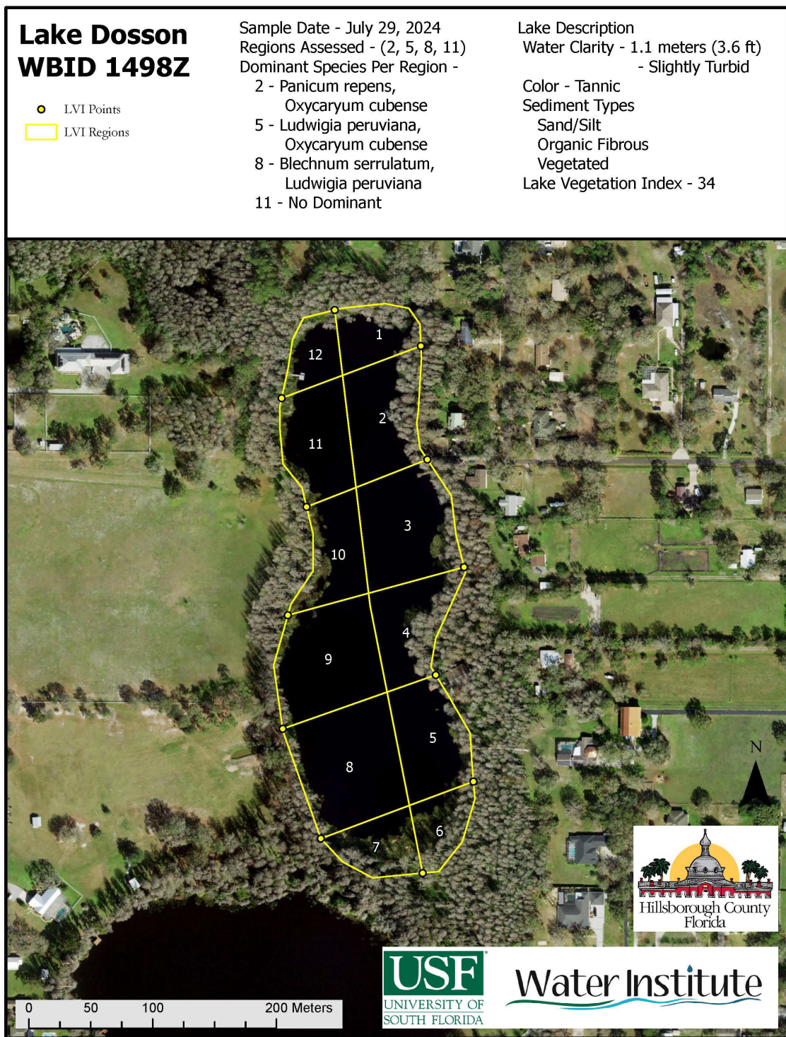
Figure 6: Lake Vegetation Index region map for Lake Dosson
