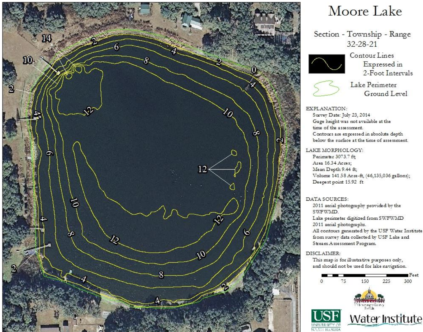
Figure 2. 2014 2-Foot Bathymetric Contour Map for Moore Lake.
