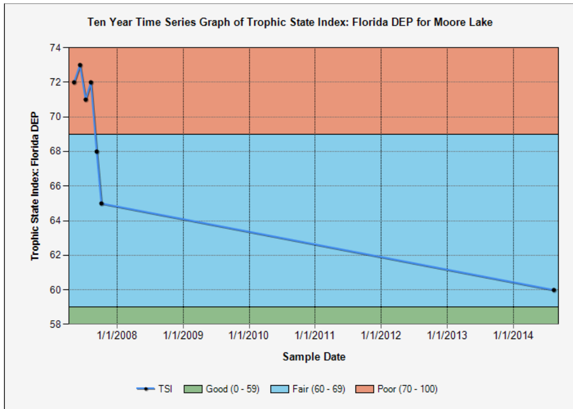
Figure 7. Recent Trophic State Index (TSI) graph for Moore Lake vi
