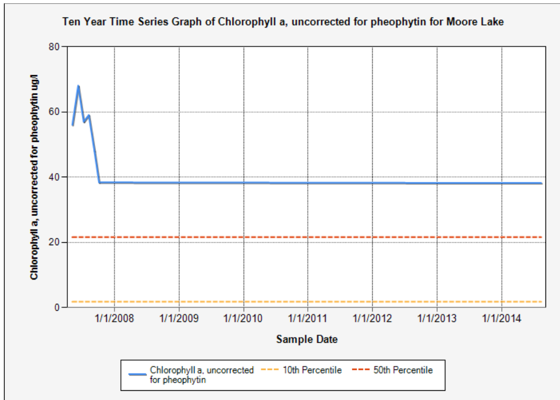
Figure 8. Recent Chlorophyll a graph for Moore Lake vii
