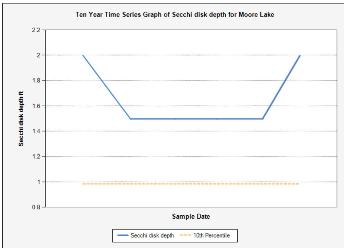
Figure 9. Recent Secchi Disk graph for Moore Lake viii
