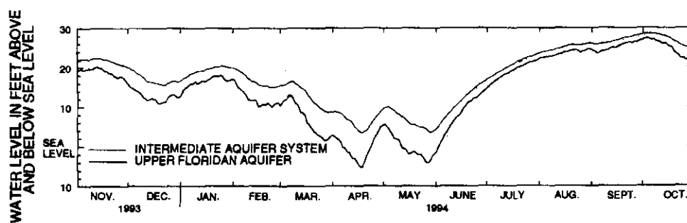
Figure 15. Seasonal flow measurements for Utopia No. 1 well in Sarasota County and hydrographs of the intermediate aquifer system and the Upper Floridan aquifer, November 1993 through October 1994.
