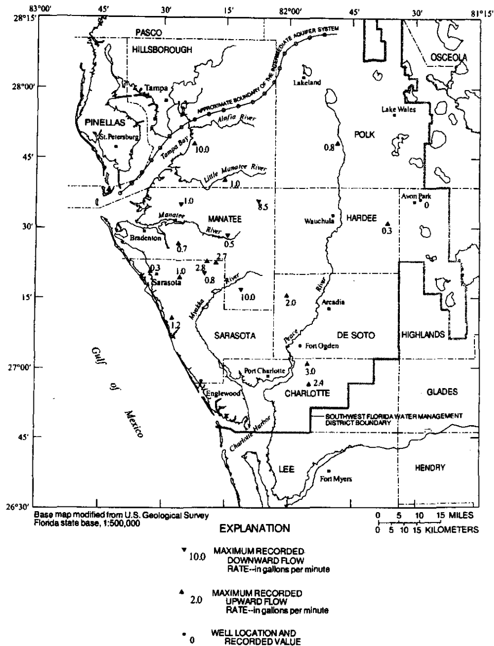
Figure 17. Locations of wells measured with the heat-pulse flowmeter and the maximum recorded flow measurement in the borehole in gallons per minute.
