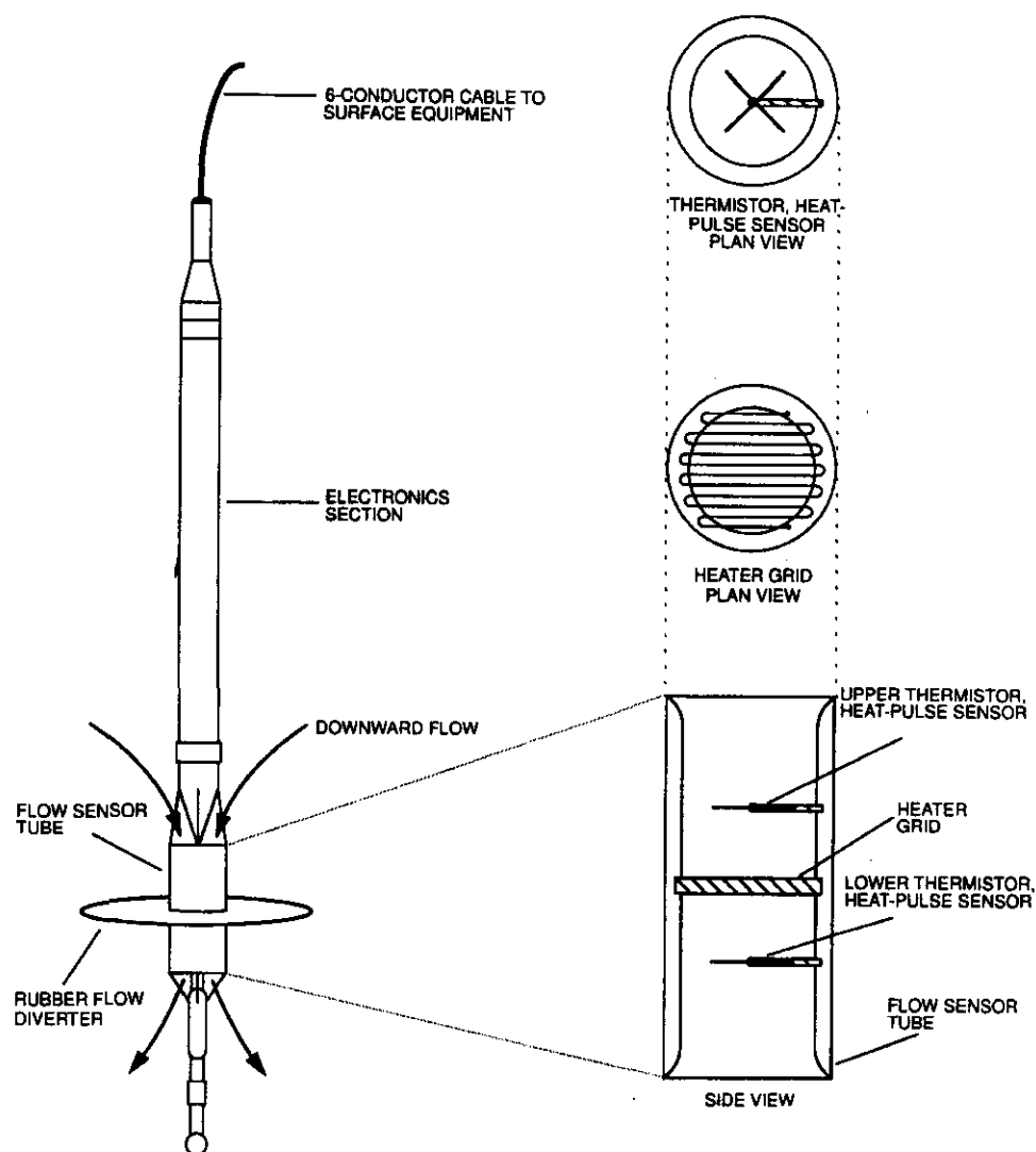
Figure B. The components of the heat-pulse flowmeter (modified from Hess, 1990).
