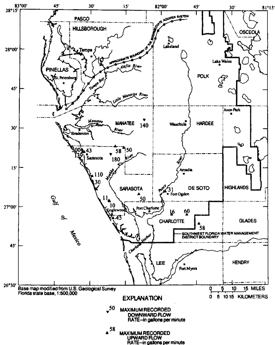
Figure 10. Locations of wells in which internal flow was detected using the impeller flowmeter and the maximum recorded borehole flow in gallons per minute.
