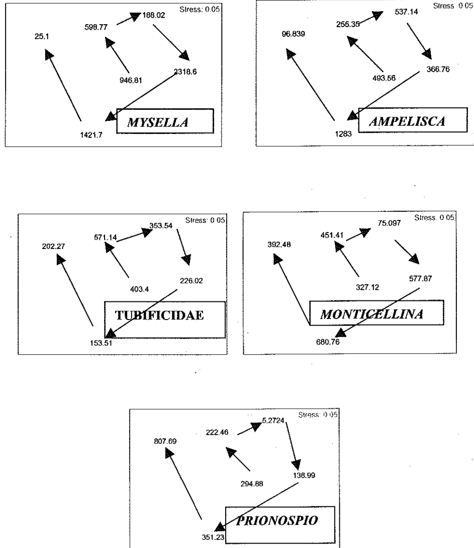
Figure 36. Mean densities (# m -2 ) concentrations of Mysella planulata , Ampelisca holmesi , tubificid oligochaetes (genera undetermined), Monticellina dorsobranchialis , and Prionospio perkinsi , in Hillsborough Bay, 1993-1998.
