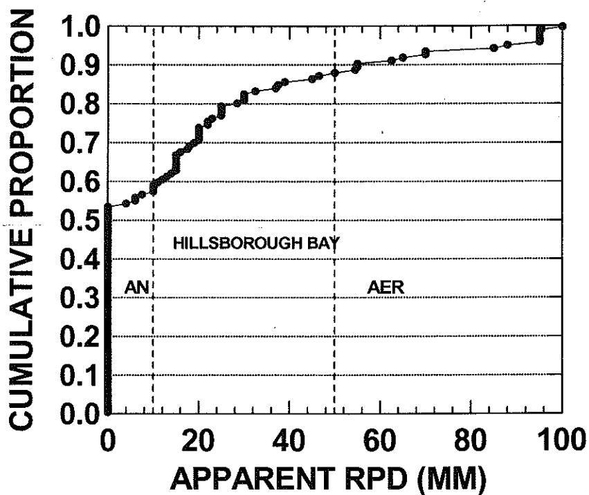
Figure 11. CDF of apparent redox potential discontinuity layer [RPD] in Hillsborough Bay, 1993-1998. Anaerobic [AN] sediments are characterized by an RPD <10-mm and aerobic [AER] sediments are characterized by an RPD >50-mm.
