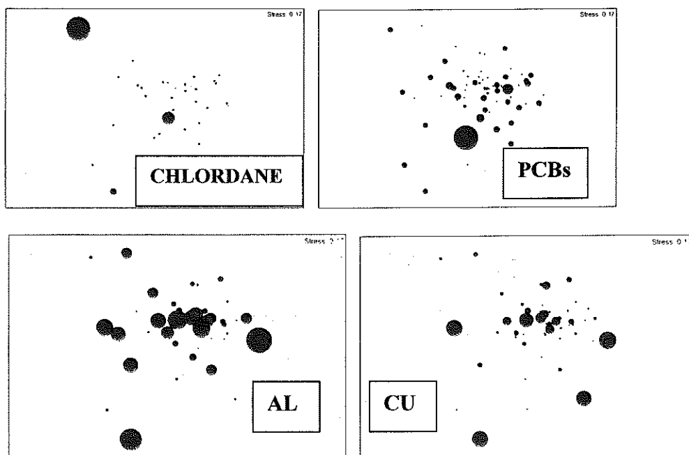
Figure 34. “Bubble” plots of chlordanes, PCBs, AL, and Cu concentrations superimposed over the MDS plot depicting benthic community structure, by year, in Hillsborough Bay 1995-1998
