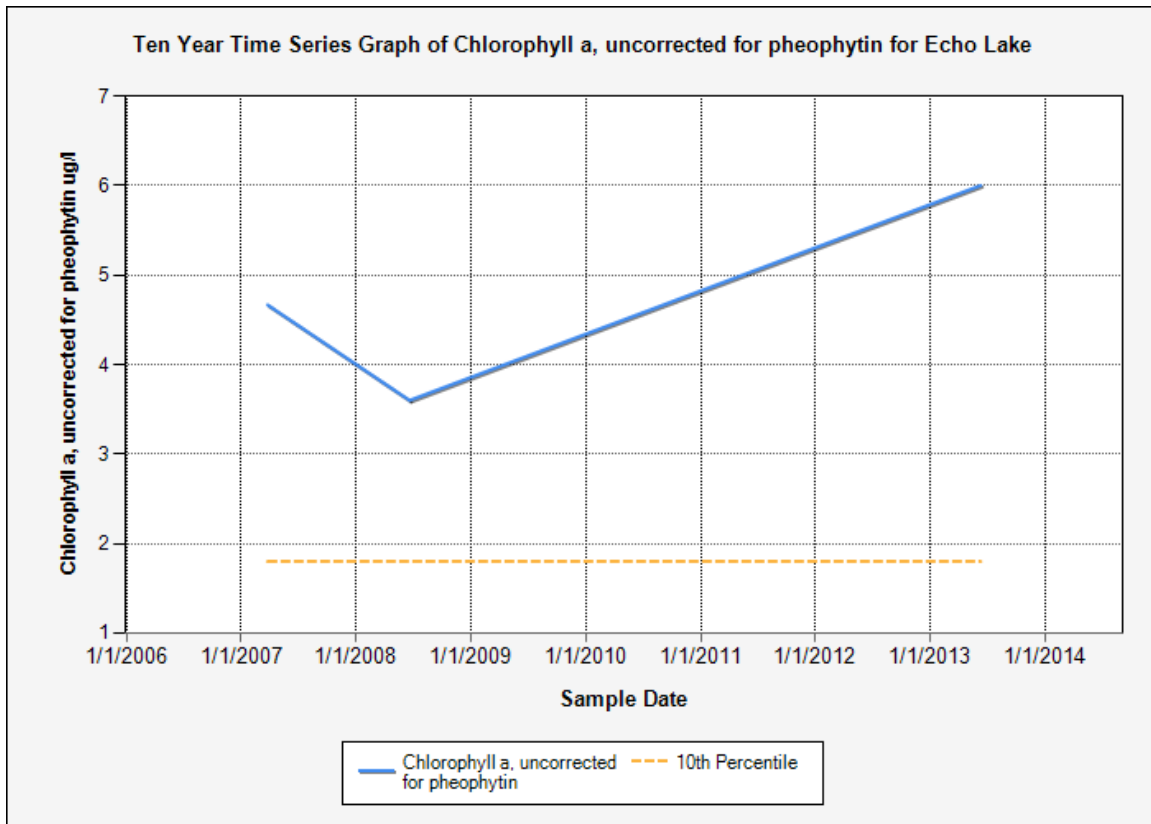
Figure 8. Recent Chlorophyll a graph for Echo Lake vii
