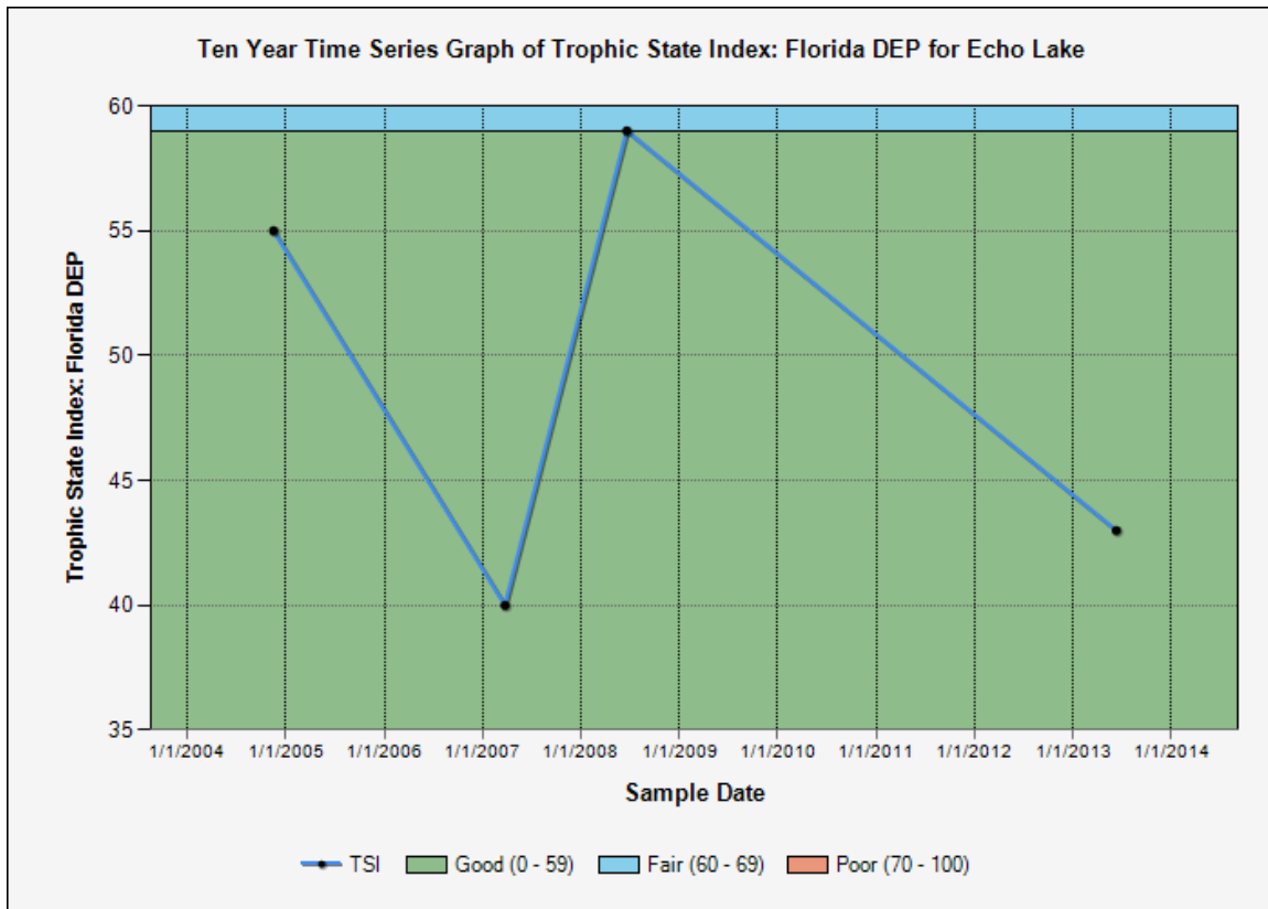
Figure 7. Recent Trophic State Index (TSI) graph for Echo Lake vi
