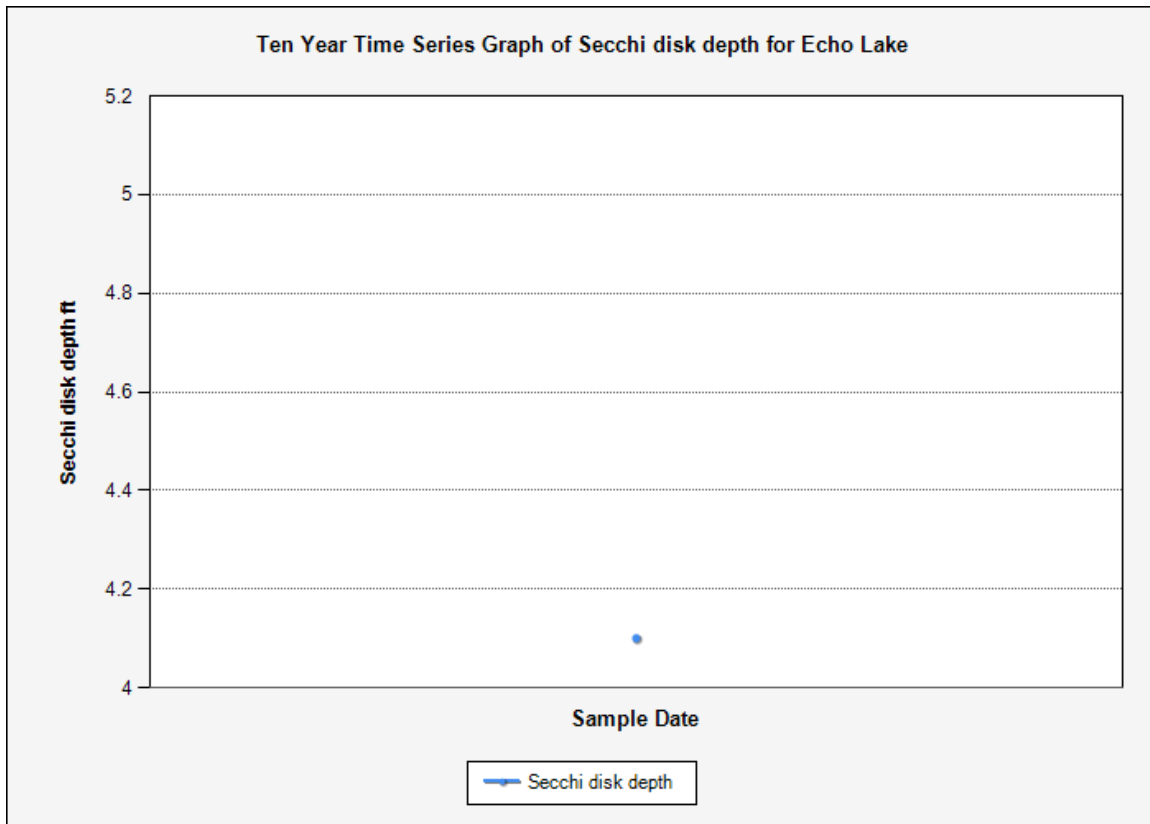
Figure 9. Recent Secchi Disk graph for Echo Lake viii
