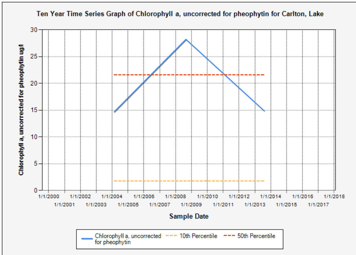
Figure 8. Recent Chlorophyll a graph for Lake Carlton vii
