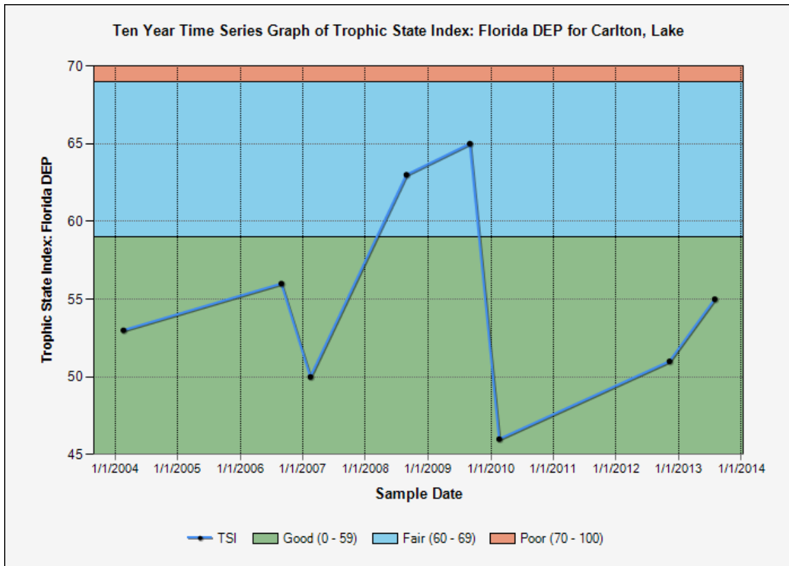
Figure 7. Recent Trophic State Index (TSI) graph for Lake Carlton vi
