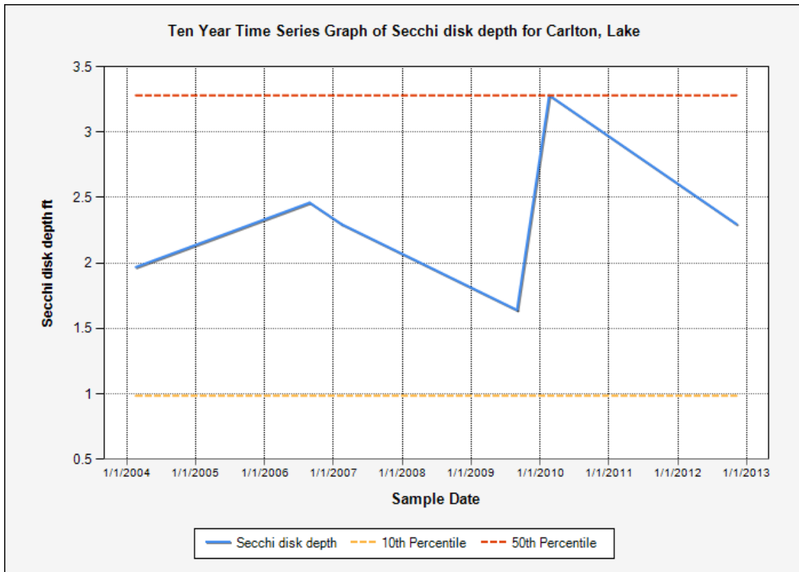
Figure 9. Recent Secchi Disk graph for Lake Carlton viii
