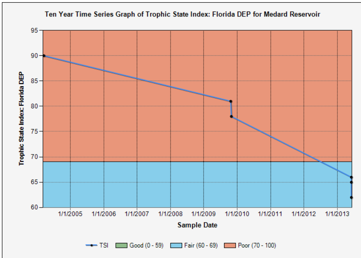
Figure 7. Recent Trophic State Index (TSI) graph for Medard Reservoir vi
