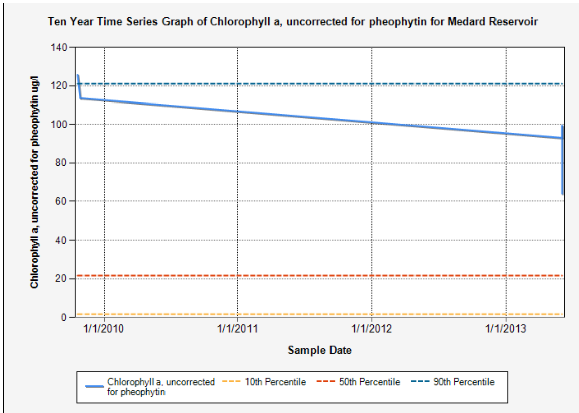
Figure 8. Recent Chlorophyll a graph for Medard Reservoir vii
