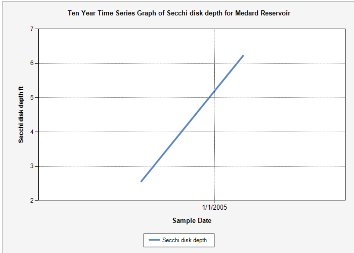
Figure 9. Recent Secchi Disk graph for Medard Reservoir viii
