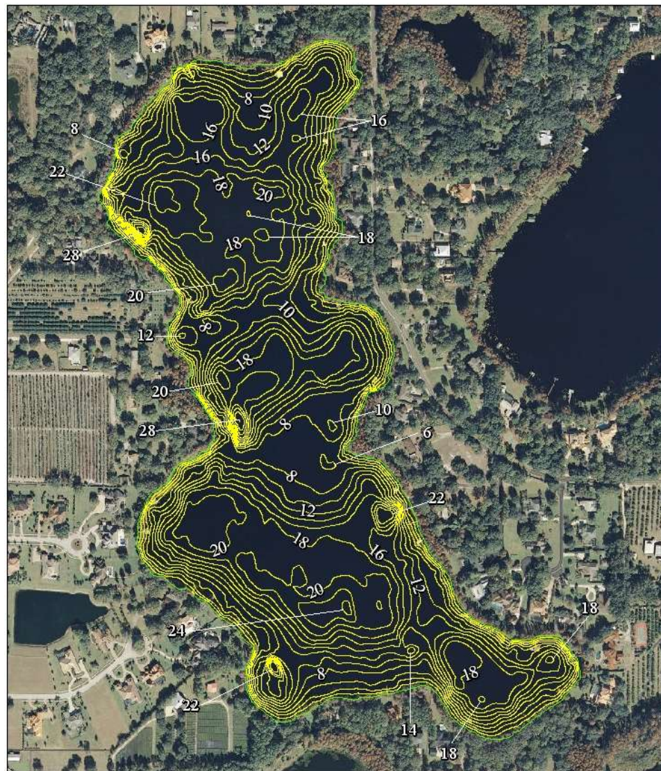
Figure 2. 2011 2-Foot Bathymetric Contour Map for Pretty Lake
