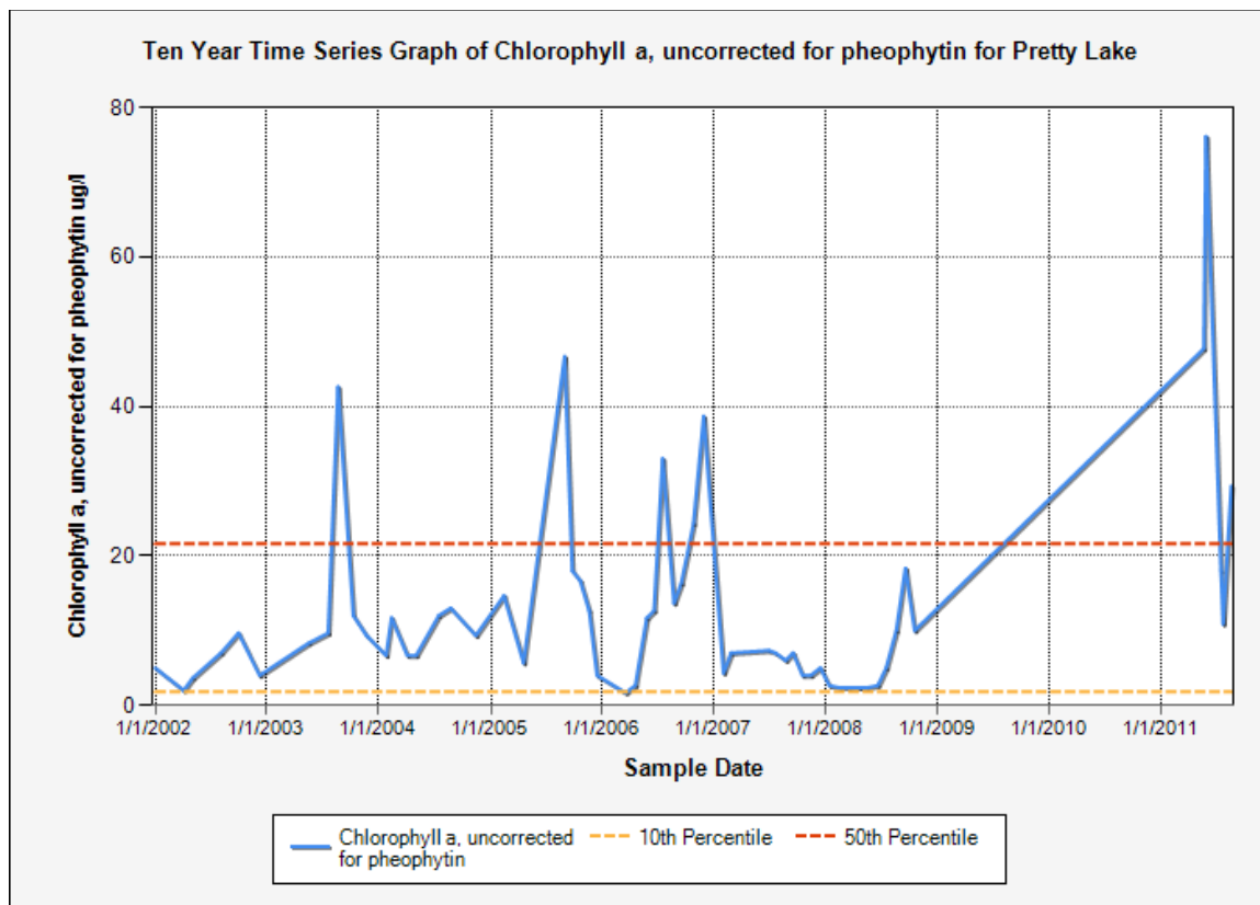
Figure 8. Recent Chlorophyll a graph for Pretty Lake vii
