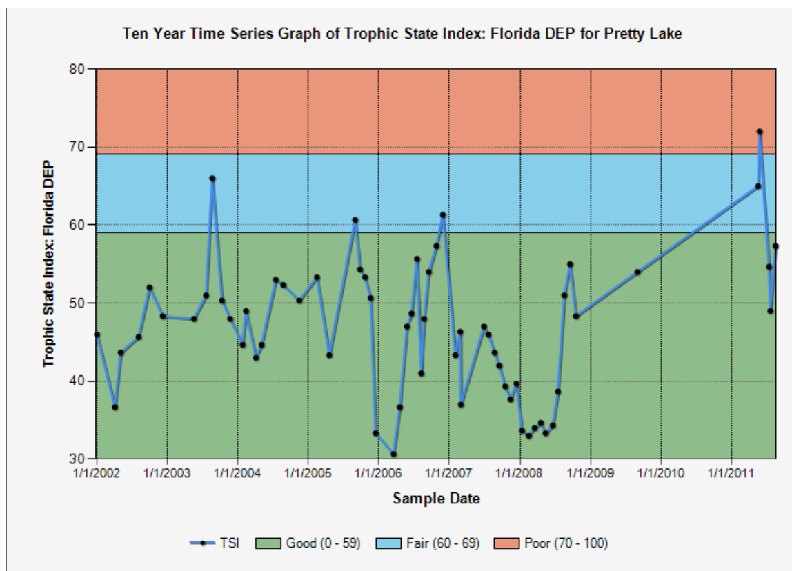
Figure 7. Recent Trophic State Index (TSI) graph for Pretty Lake vi
