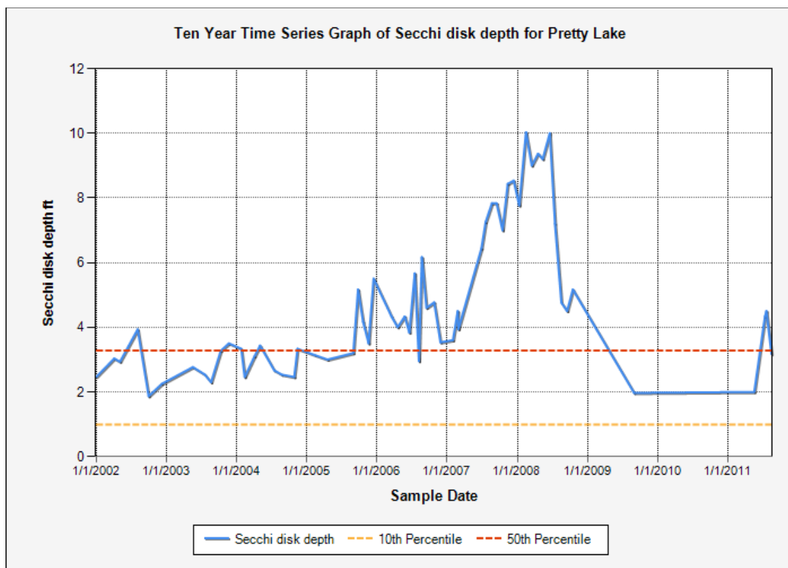
Figure 9. Recent Secchi Disk graph for Pretty Lake viii
