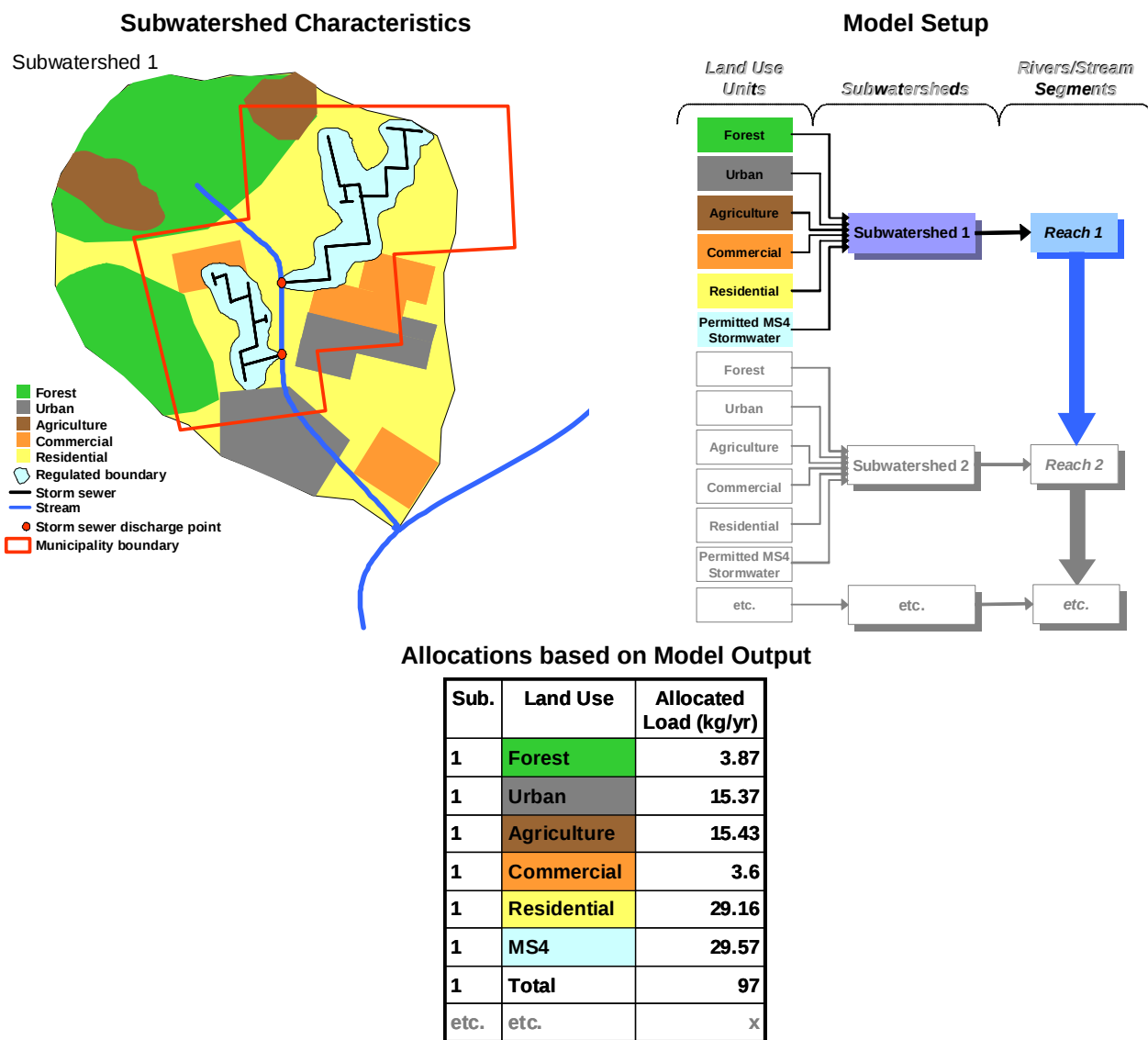
Figure 17. Process for calculating MS4 allocation when the MS4 drainage area is included in the model as a discrete land unit.
