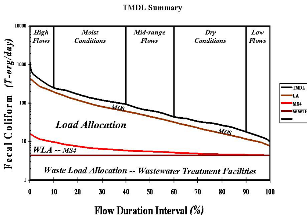
Figure 19. Example TMDL using duration curve framework
